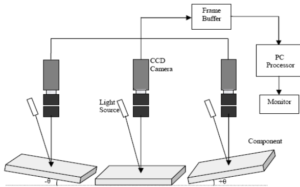
Fig. 2 Schematic diagram of the machine vision system.
