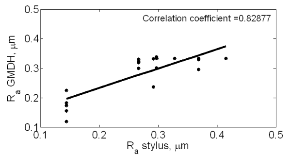
Fig. 3 Relationship between calculated R_a values using GMDH and stylus R_a values.
